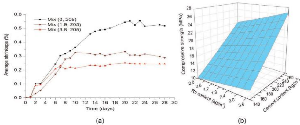
Figure 13. (a) Effect of synthetic zeolite on shrinkage reduction and (b) on SCS gain as a function of dosage (adapted from [73]).
